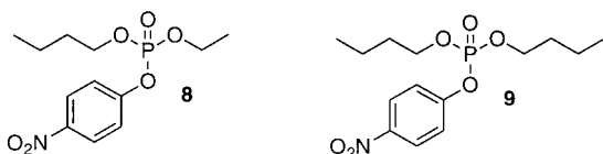
Figure 5. Compounds employed to determine specificity of hydrolytic activity by mAb 1H9.
