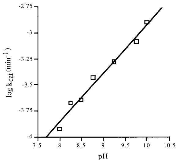
Figure 4. Dependence of \log k_{\text{cat}} antibody 1H9 catalyzed paraoxon hydrolysis on pH.
