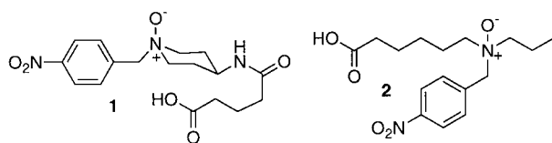
Figure 3. The constrained hapten 1 , previously employed to obtain antibody catalysts for the hydrolysis of paraoxon, and the more flexible hapten 2 used in the current study.
