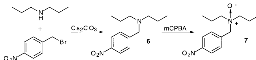
Scheme 2. Synthesis of hapten analogue 7 used to determine K_i with mAb 1H9.
