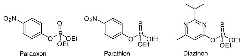
Figure 1. Representative phosphotriester insecticides.
