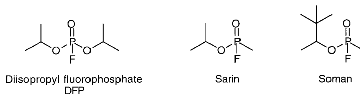
Figure 2. Representative G-series nerve agents and their surrogates.
